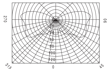
Luminous intensity distribution cd/1000lm
